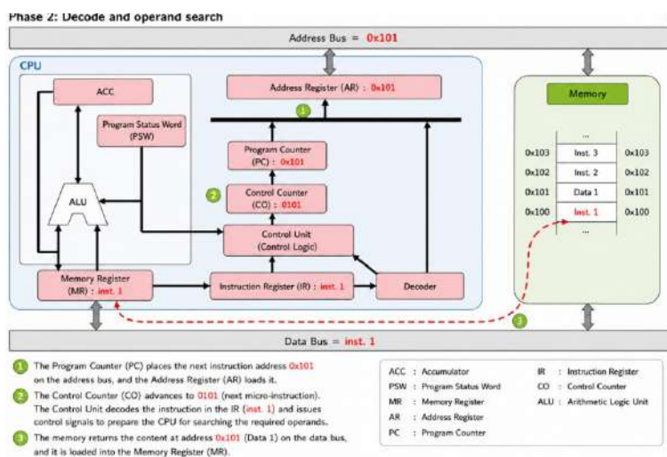
Figure III. 4 - Decode Phase (Instruction Decoding and Operand Retrieval)
